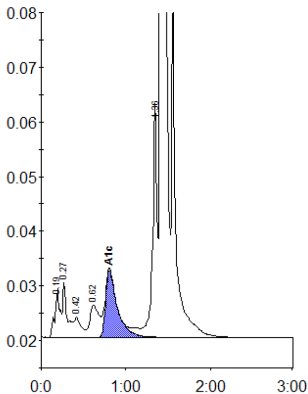
Peak table - ID: 10646823
